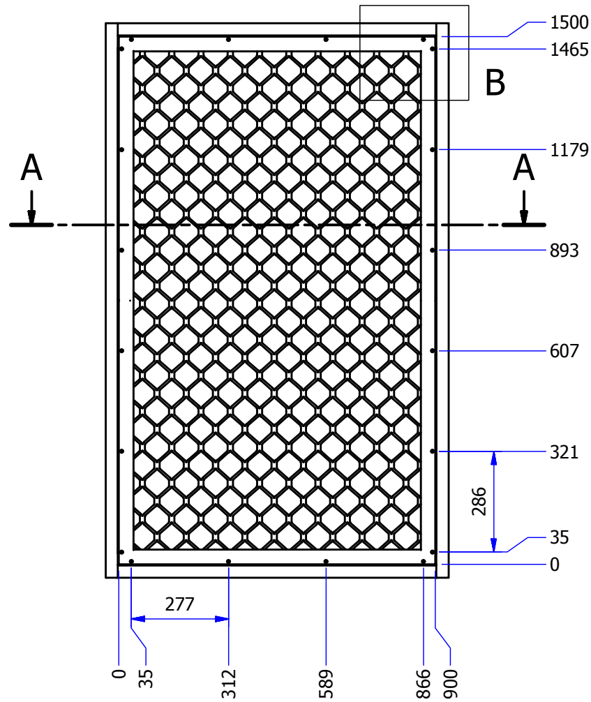
FRONT VIEW 1 ( 1 : 15 )
