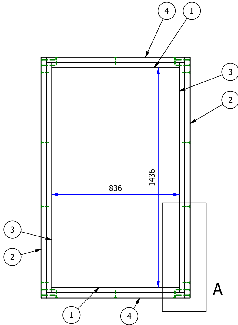
FRONT VIEW 1 ( 1 : 15 )
